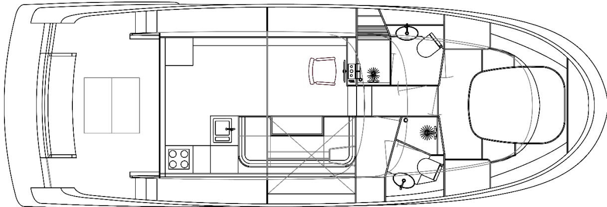
Steeler NG43S Layout with optional second bathroom
